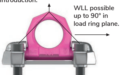
VRBG split force introduction.
