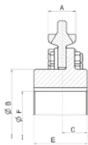
Sprocket wheel multi-part **
