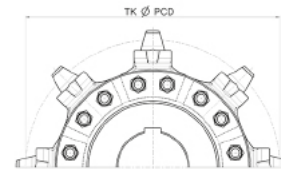
Sprocket wheel multi-part **
