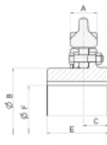
Sprocket wheel multi-part*
